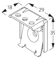
SG 8201 Bracket
