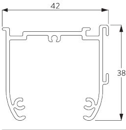
SG 2321 Profile
