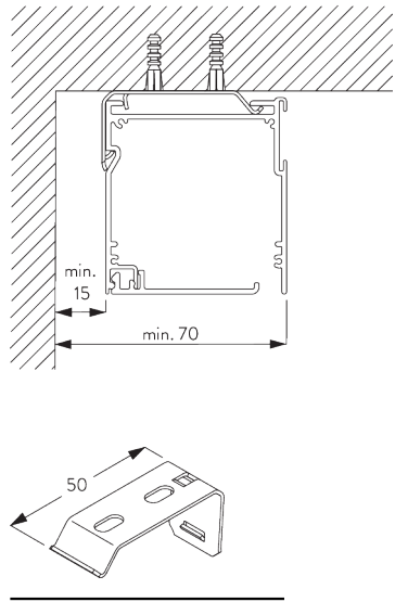
SG 2521 Bracket
