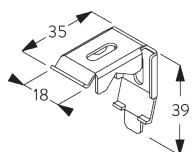
SG 2302 Bracket
