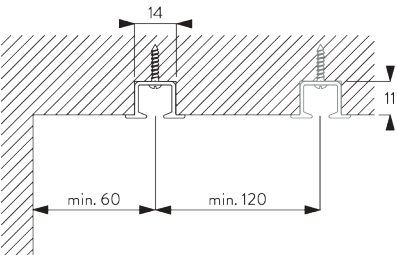
Recess channel: 11 x 14 mm
