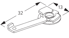
SG 3060 Clamp
