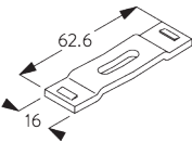
SG 3113 Bracket
